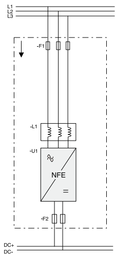
NFE Non-regenerative front-end
