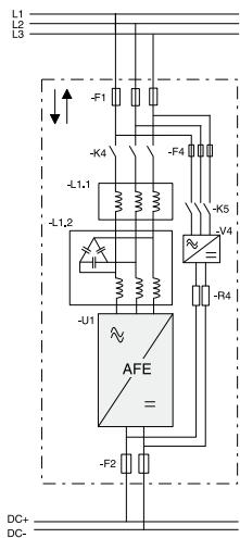
AFE Active front-end
