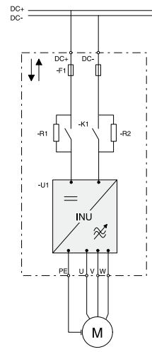
INU Inverter Unit (FI9-FI14)
