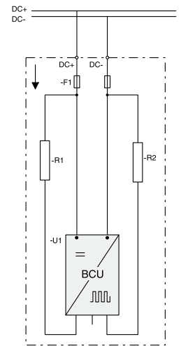
BCU Brake chopper unit
